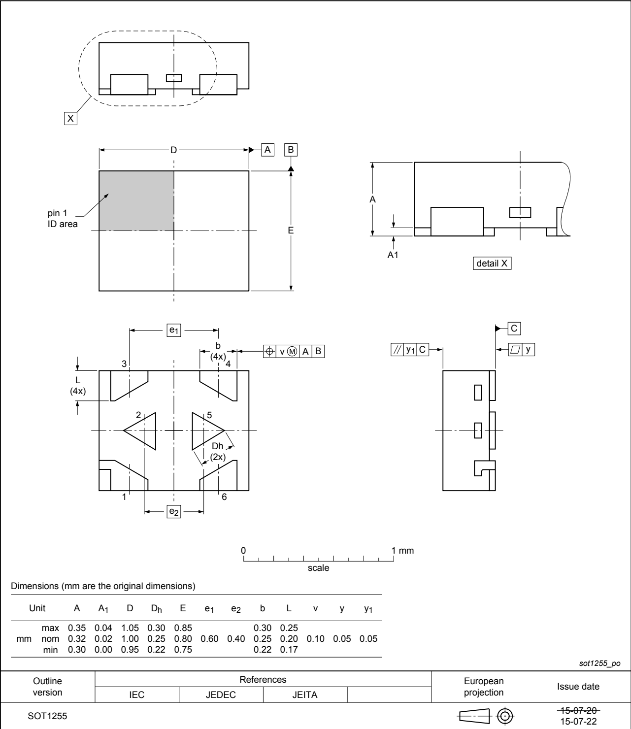
Figure 17. Package outline SOT1255 (X2SON6)
